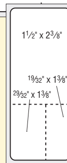
THERM-389R 3 3/4" x 1 1/2"
